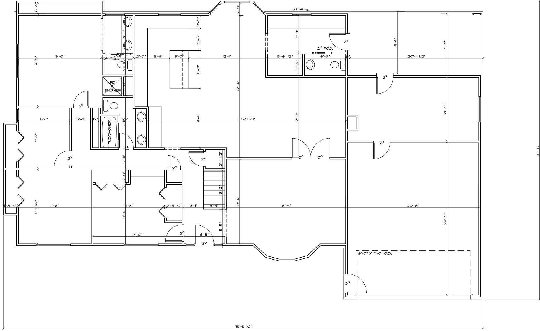
EXISTING MAIN FLOOR PLAN SCALE 1/4"
